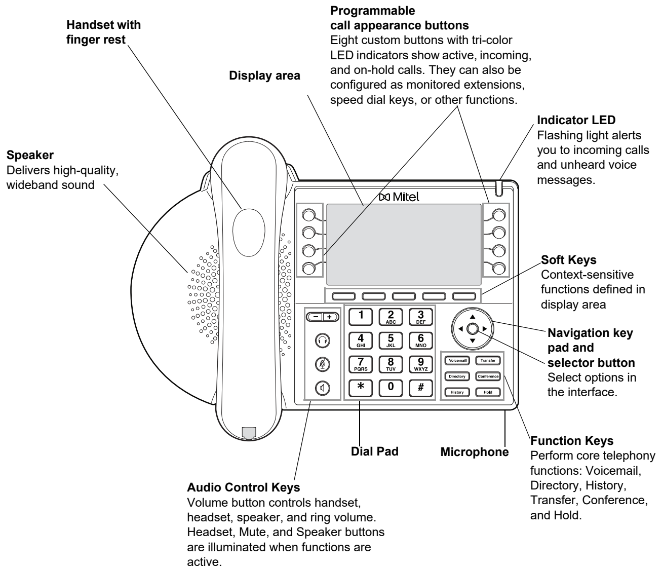
Figure 1: IP Phone 480/480g Components
