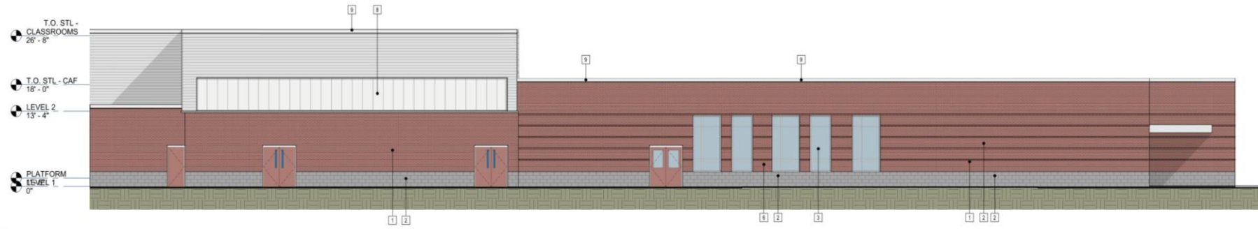
1 NORTH ELEVATION - PRESENTATION 1/8" = 1'-0"
