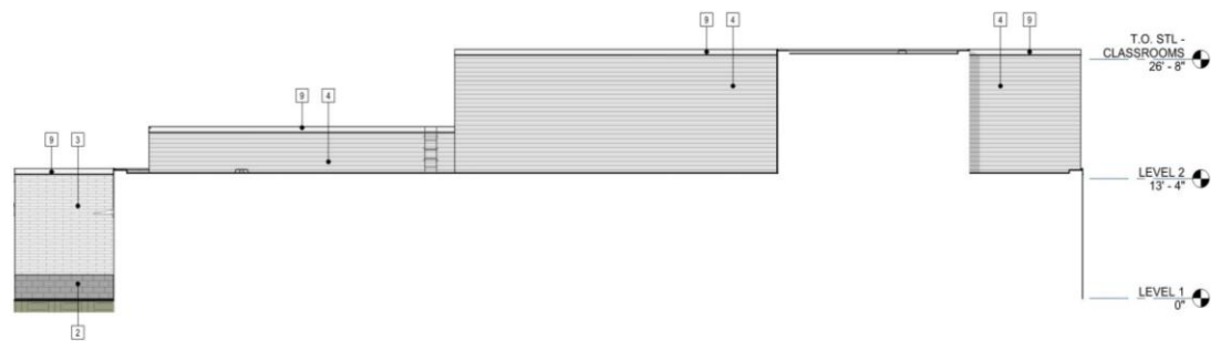
3 EAST GYM ELEVATION - PRESENTATION 1/8" = 1'-0"
