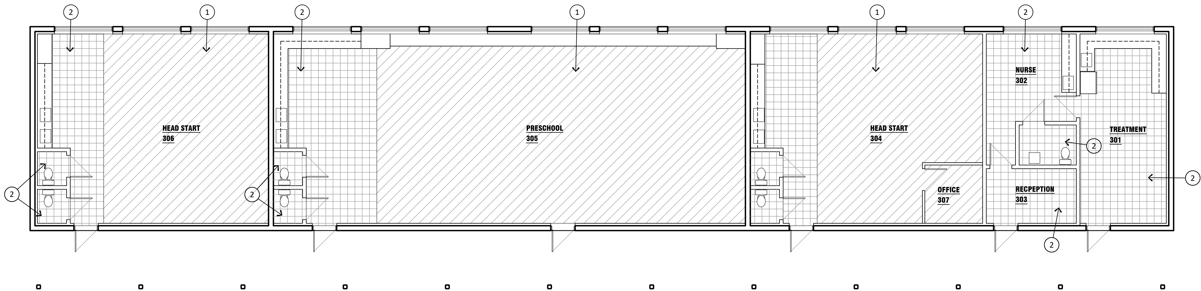
BUILDING 1300 DEMOLITION PLAN scale: 1/8" = 1'-0"
