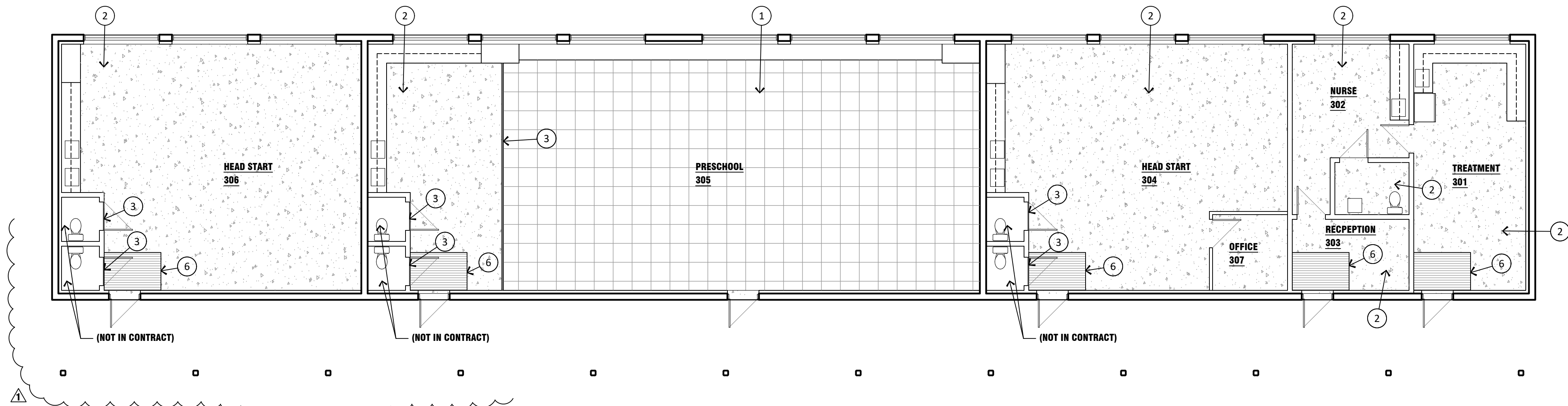
BUILDING 1300 FLOOR PLAN scale: 1/8" = 1'-0"
