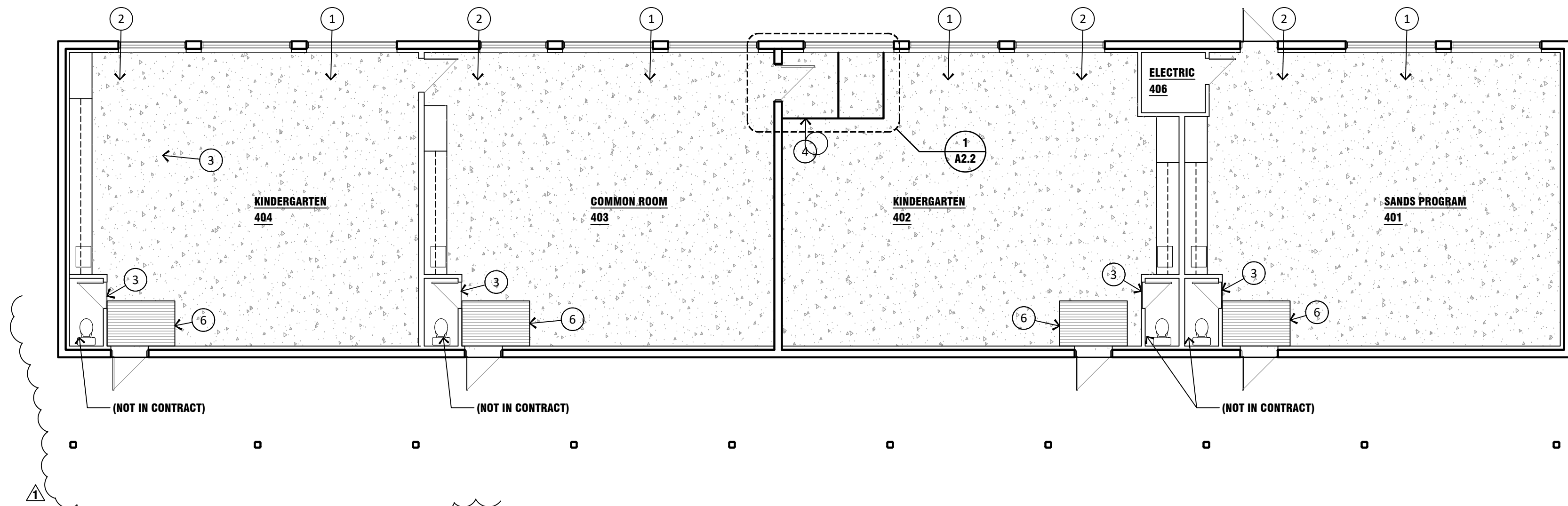
BUILDING 1400 FLOOR PLAN scale: 1/8" = 1'-0"
