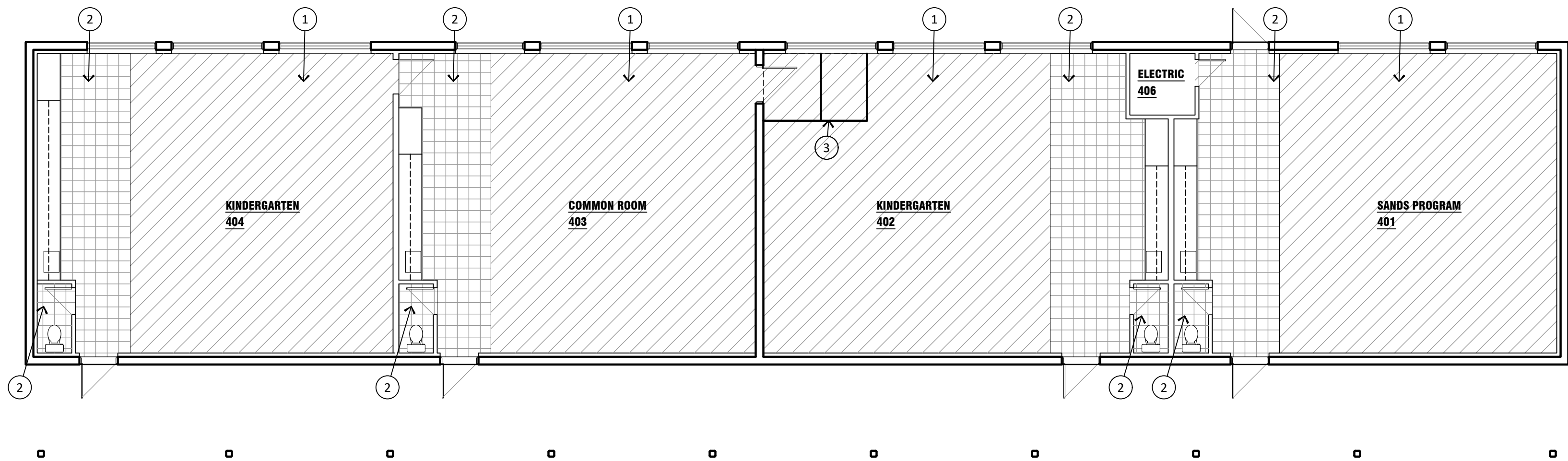
BUILDING 1400 DEMOLITION PLAN scale: 1/8" = 1'-0"
