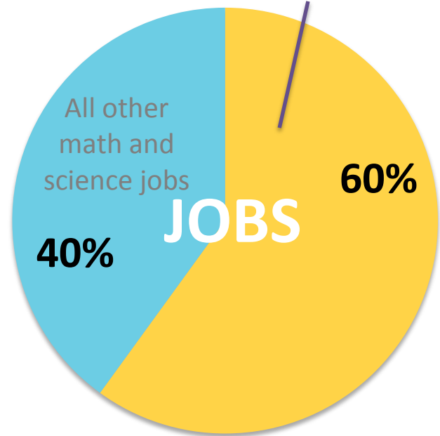
Computing Jobs
