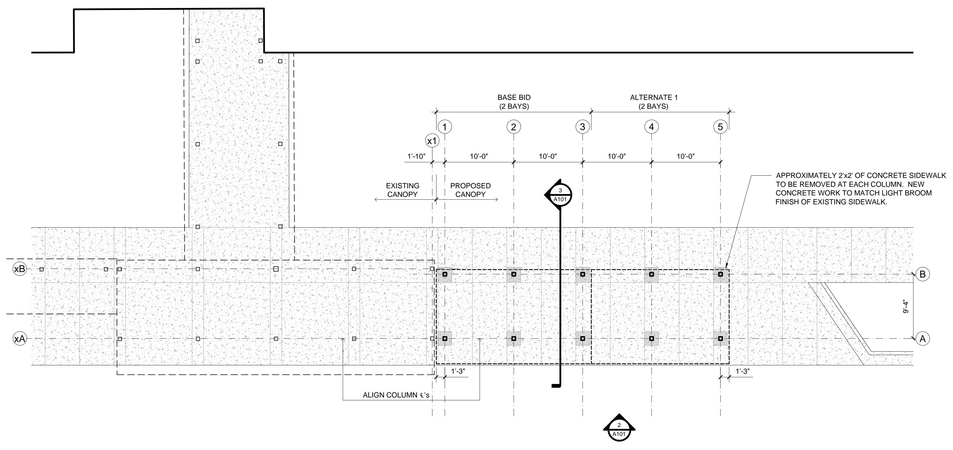
1 FLOOR PLAN 8 6 4 2 0 8 16
