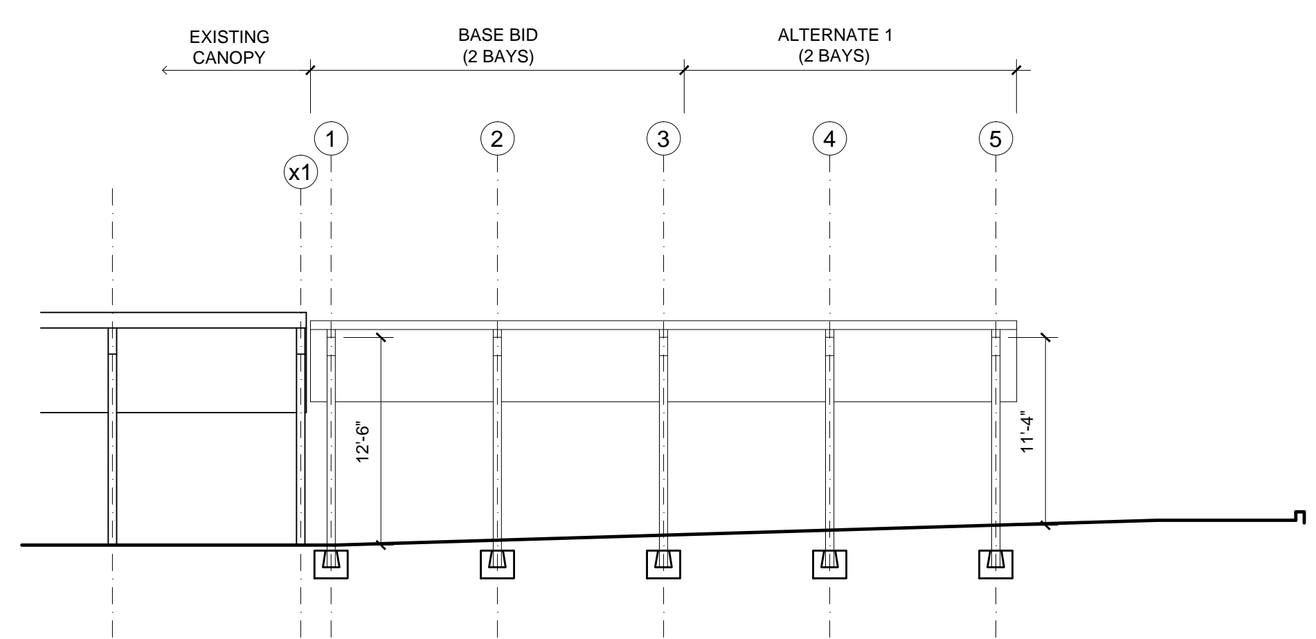
2 FRONT ELEVATION 8 6 4 2 0 8 16
