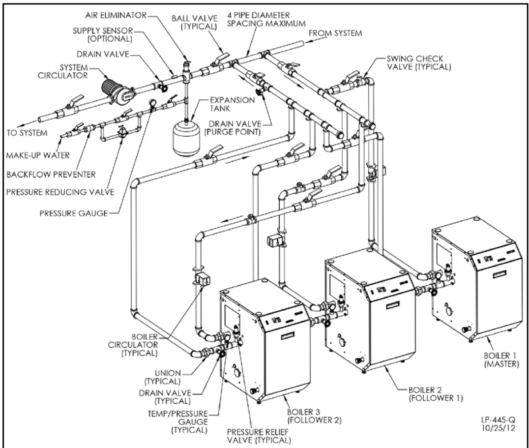
Figure 9 - Cascaded Boilers Space Heating
