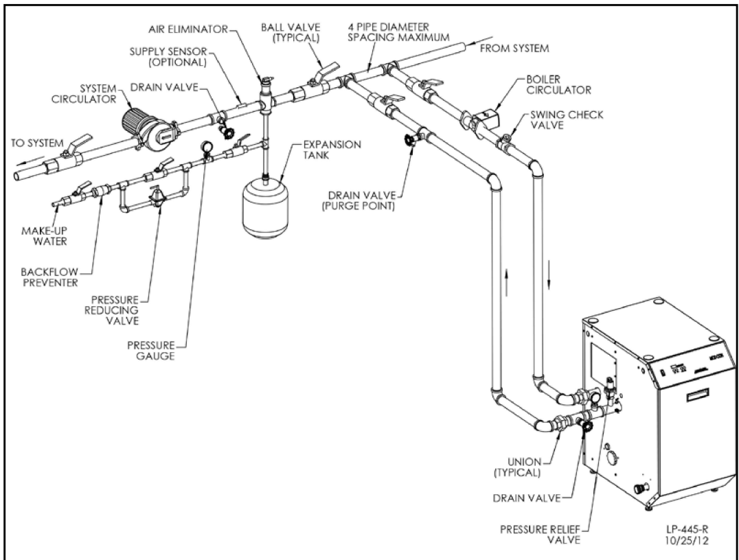
Figure 8 - Single Boiler Space Heating
