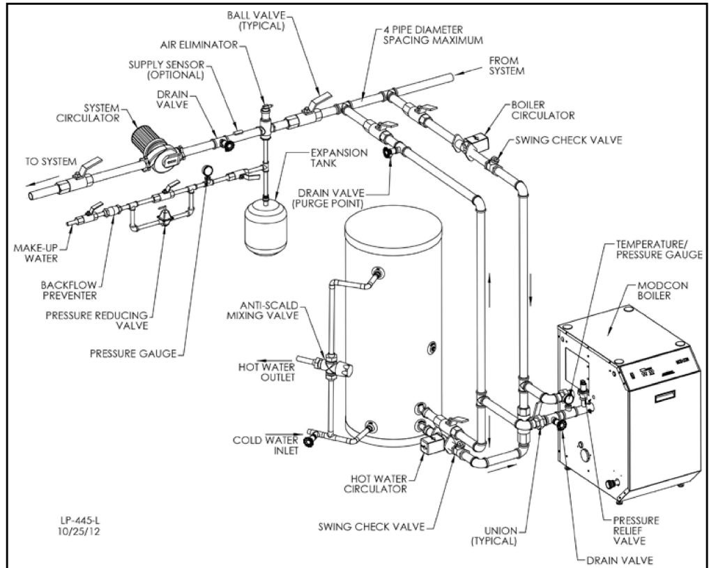
Figure 6 - Single Boiler Space Heating with Indirect Priority
