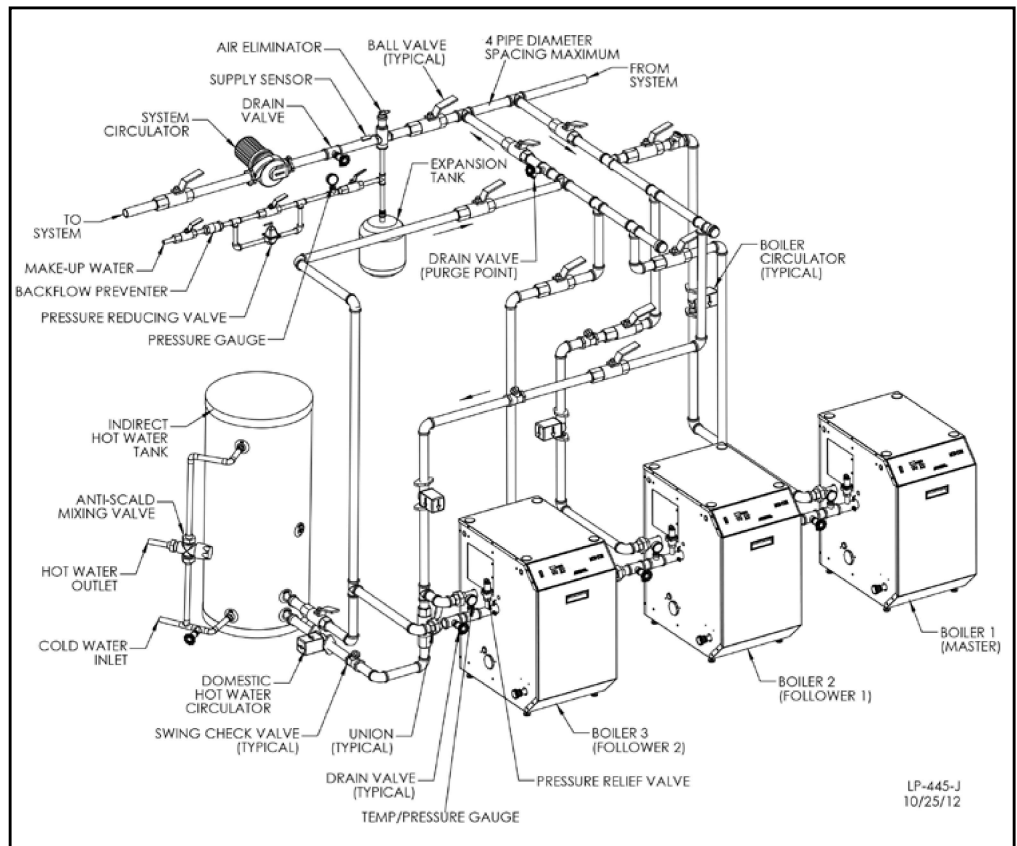
Figure 7 - Cascaded Boilers with Indirect Priority on One
