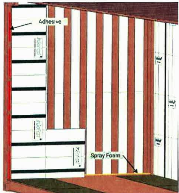
Install UX panels in a running bond pattern vertically.
