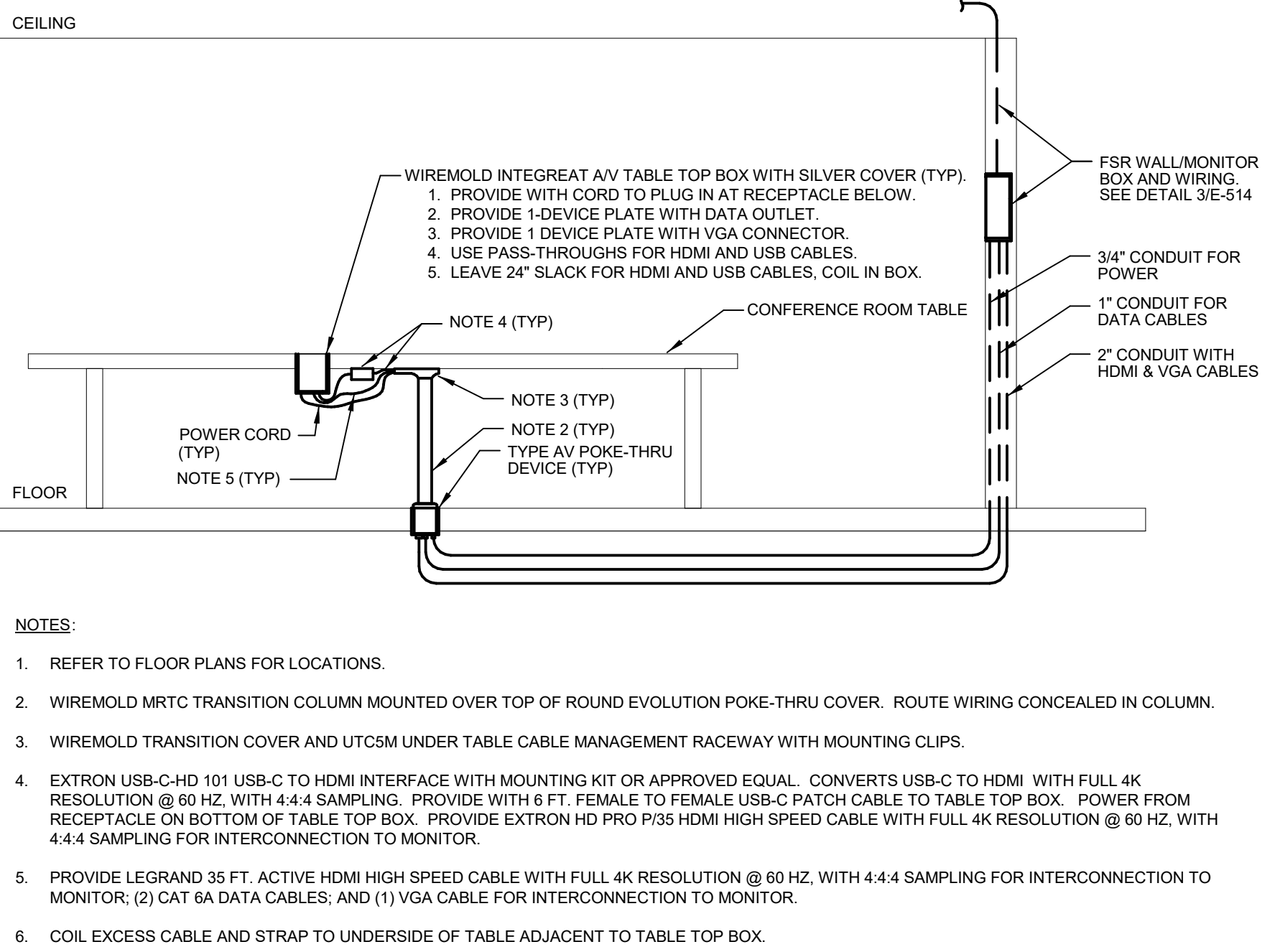
8 TYPICAL CONFERENCE ROOM POKE THRU WIRING DETAIL N.T.S.
