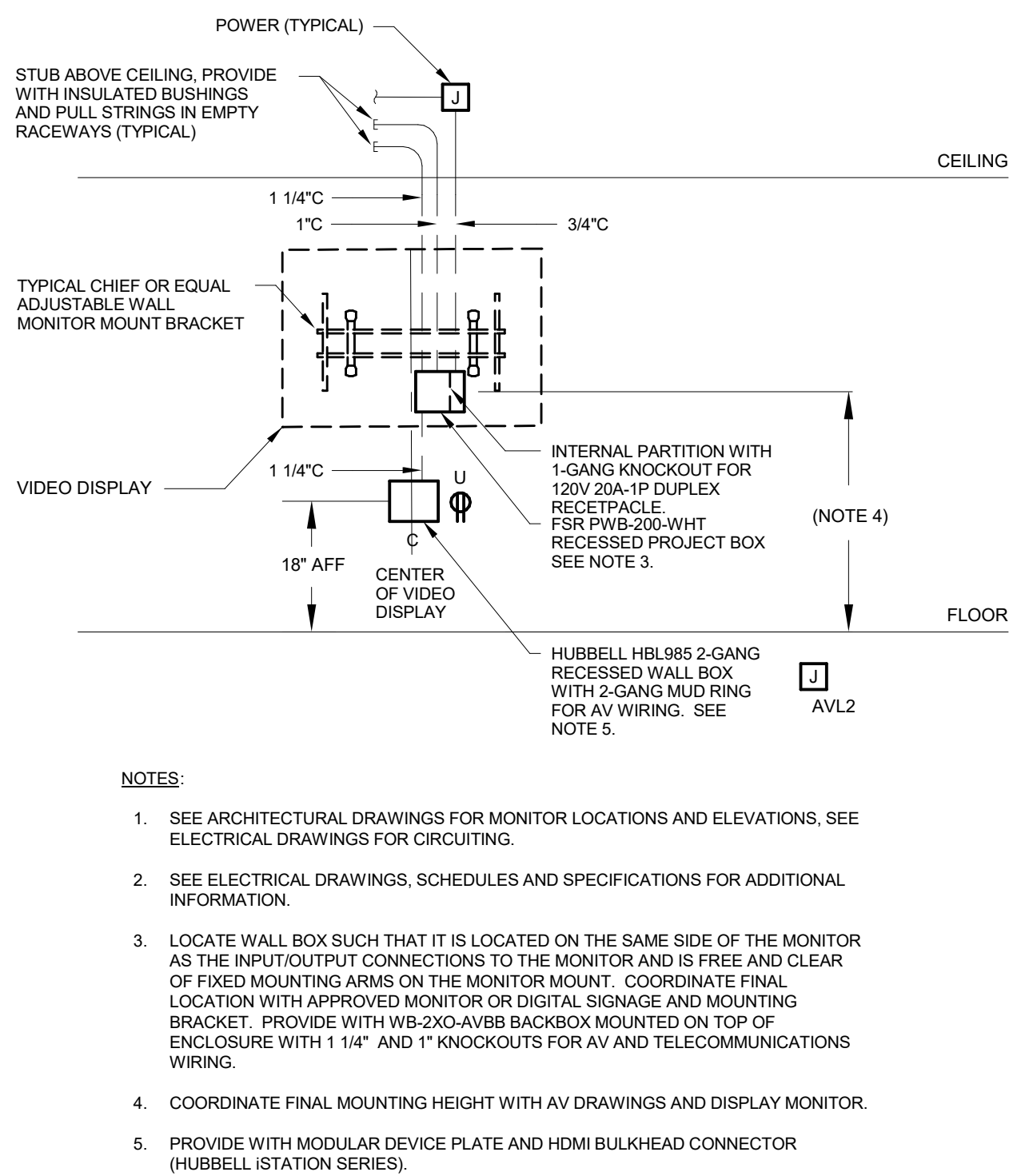
4 TYPICAL INSTRUCTIONAL MONITOR DISPLAY ROUGH-IN DETAIL N.T.S.
