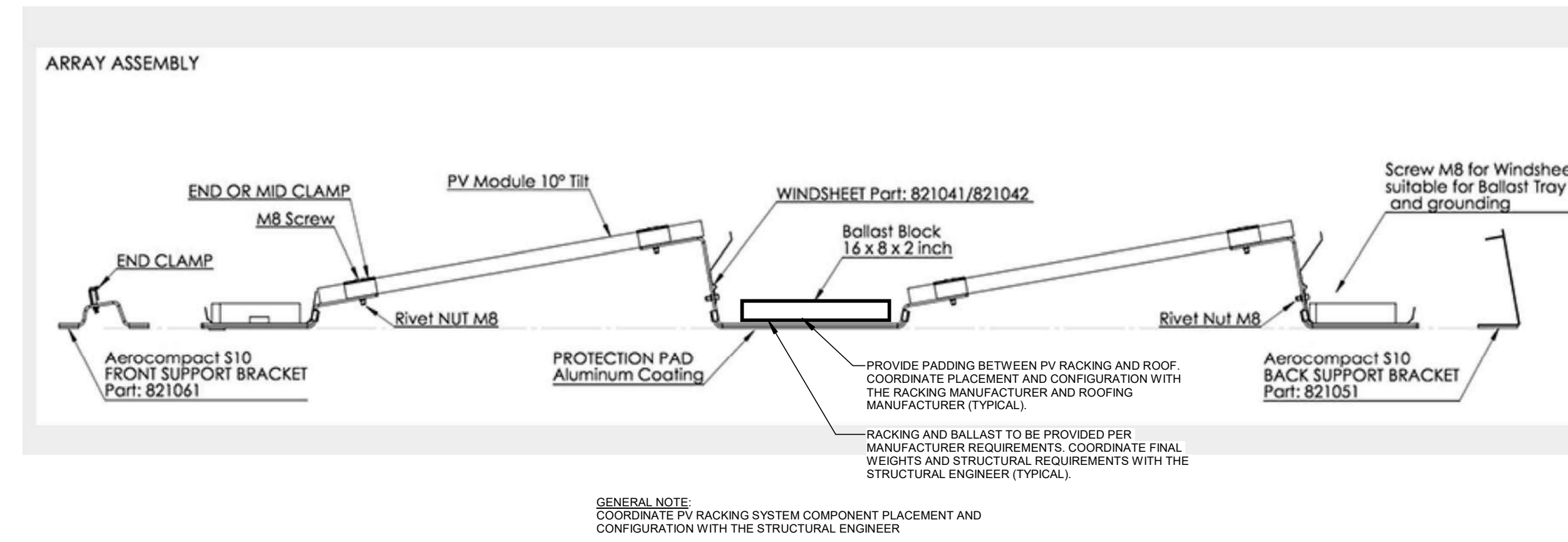
6 ROOF MOUNTED PV ARRAY DETAIL N.T.S.
