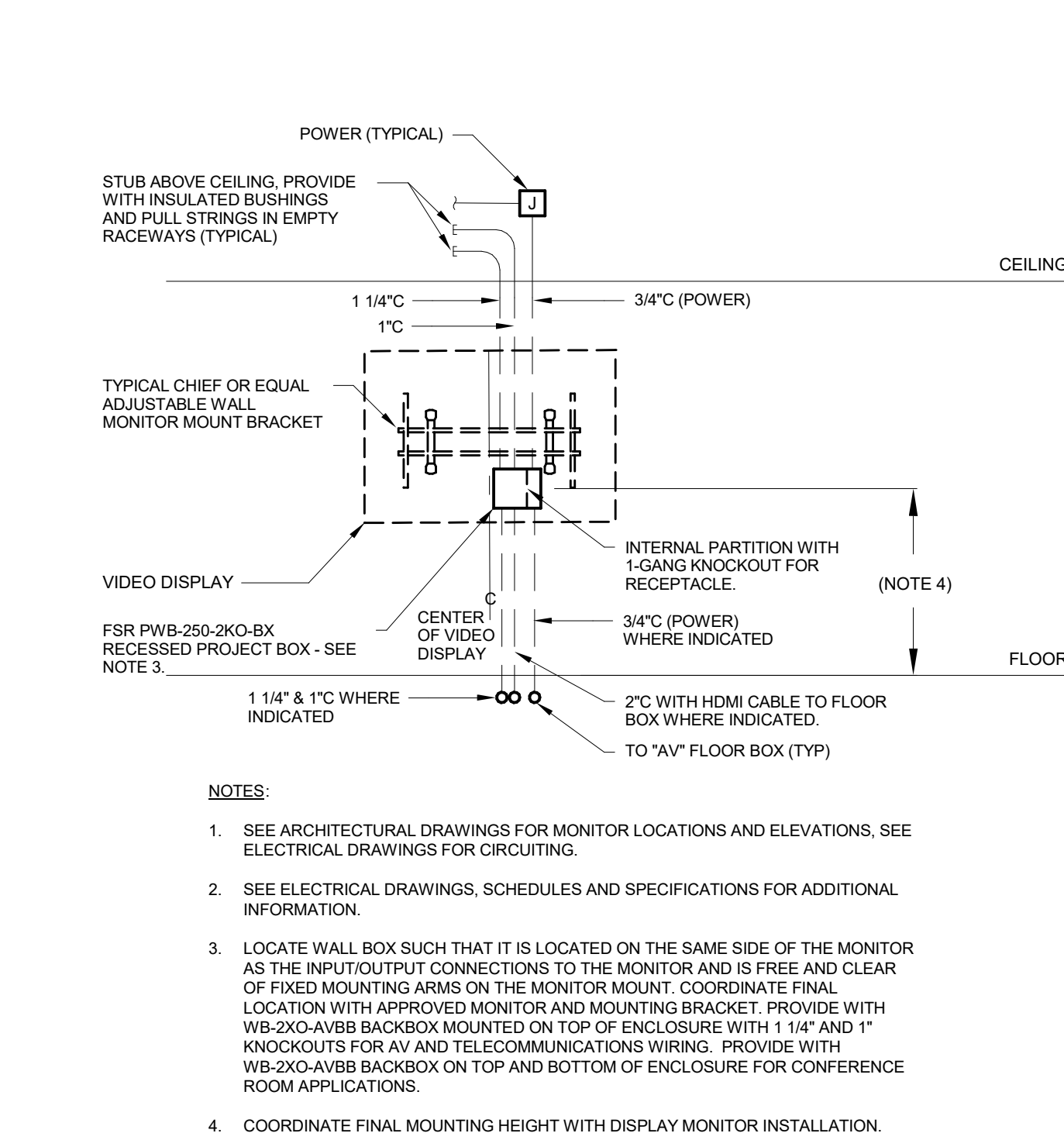
3 TYPICAL VIDEO MONITOR DISPLAY / DIGITAL SIGNAGE ROUGH-IN DETAIL N.T.S.
