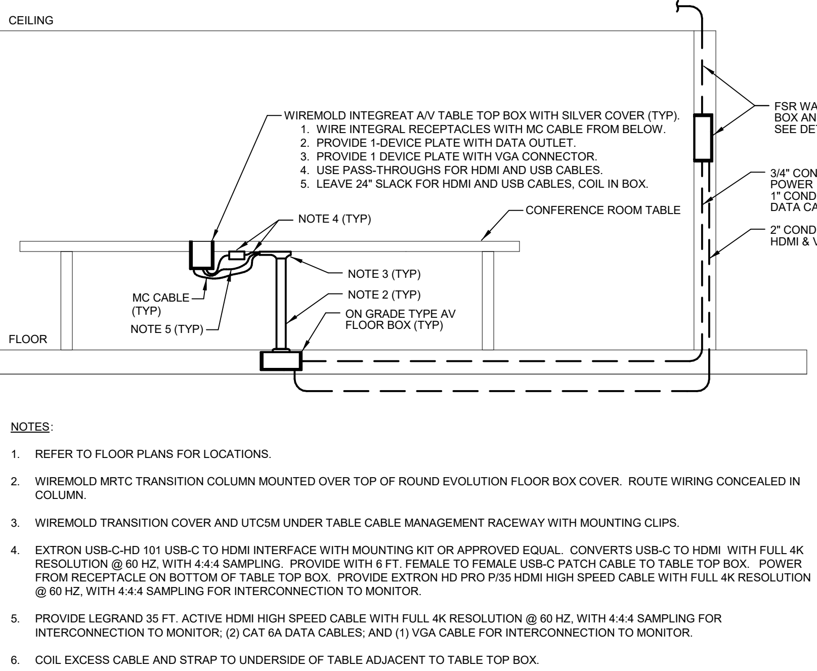
7 TYPICAL CONFERENCE ROOM ON GRADE BOX WIRING DETAIL N.T.S.
