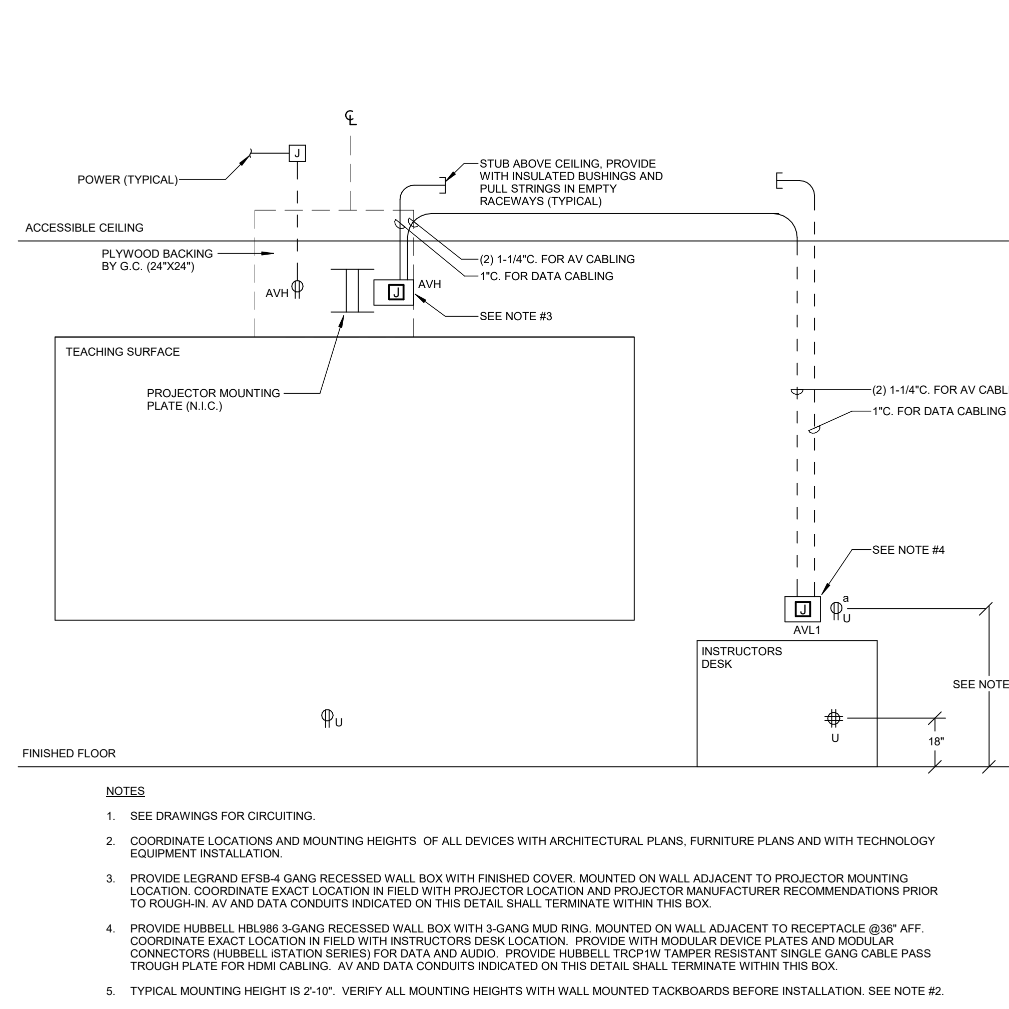
1 TYPICAL INTERACTIVE PROJECTOR ROUGH-IN DETAIL N.T.S.
