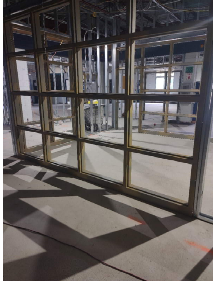
Custom borrow light hollow metal frames are set for the Small Group Rooms in Area B
