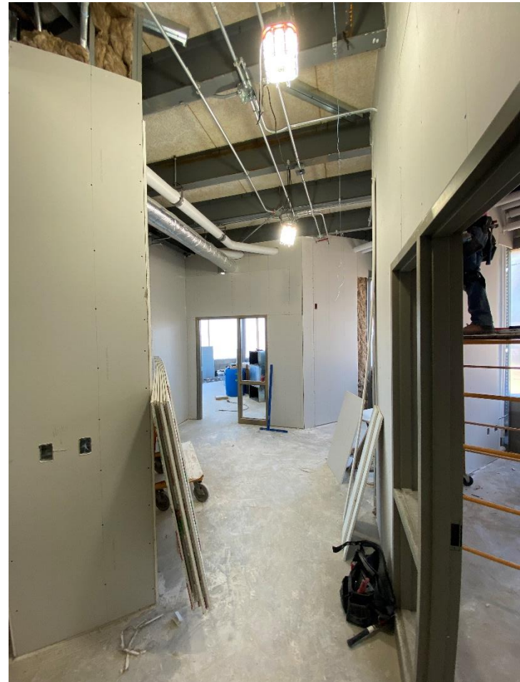
Drywall hung in new office area of secured entry addition
