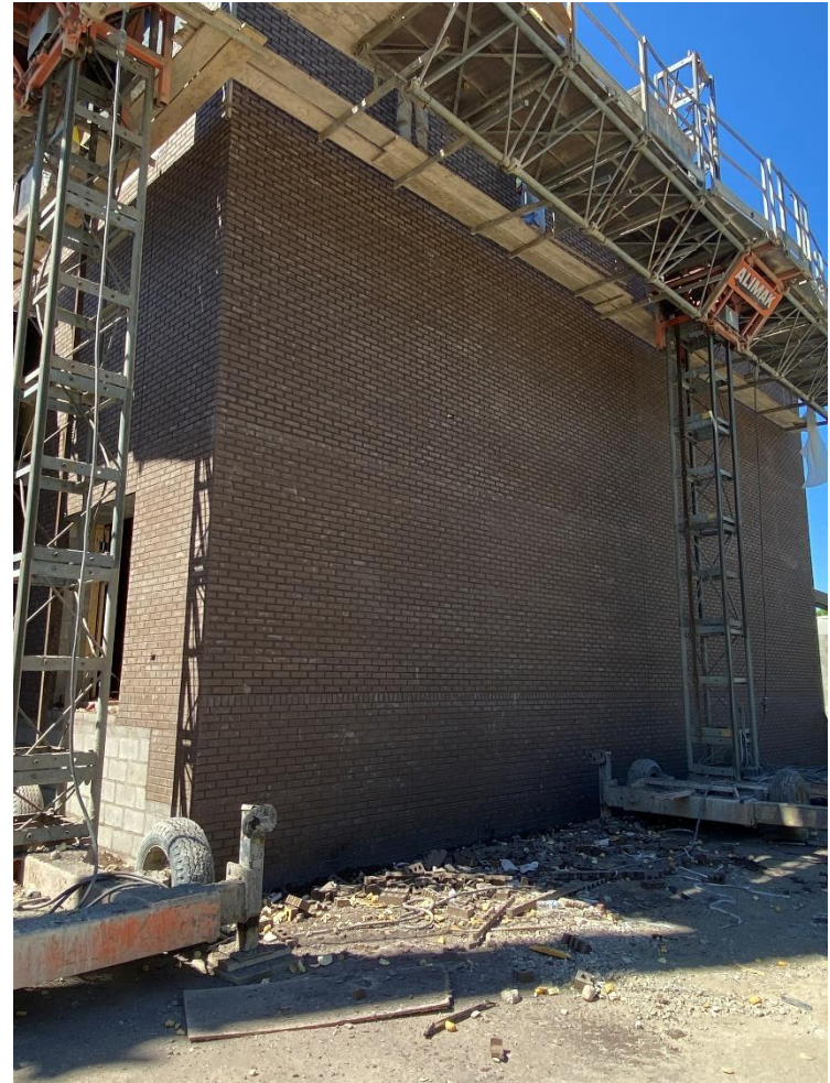
Masonry brick work on going for gym addition
