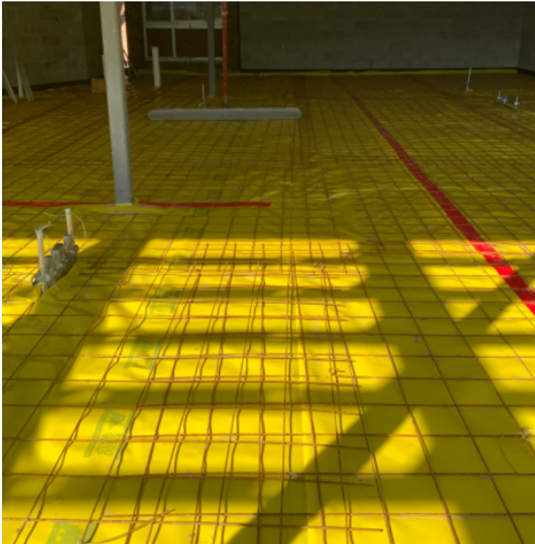
Vapor barrier and reinforcing steel are in place ahead of concrete floor slab pour
