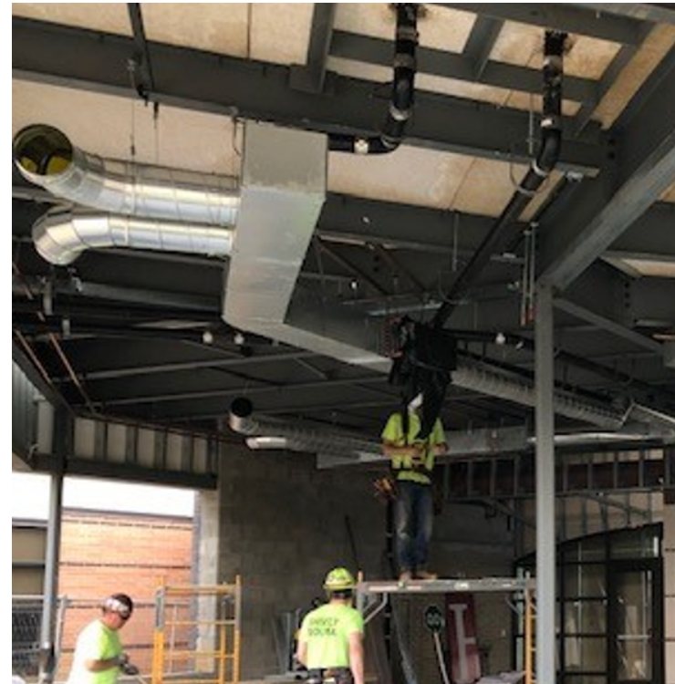
HVAC duct work being installed
