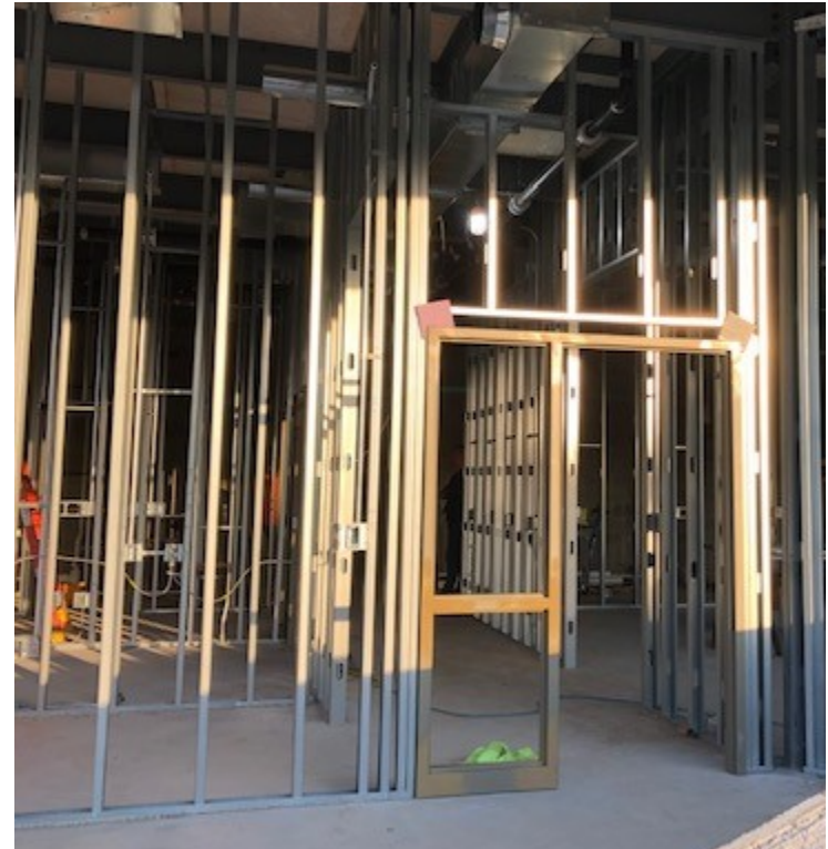
Interior metal studs and Hollow metal door frames installed
