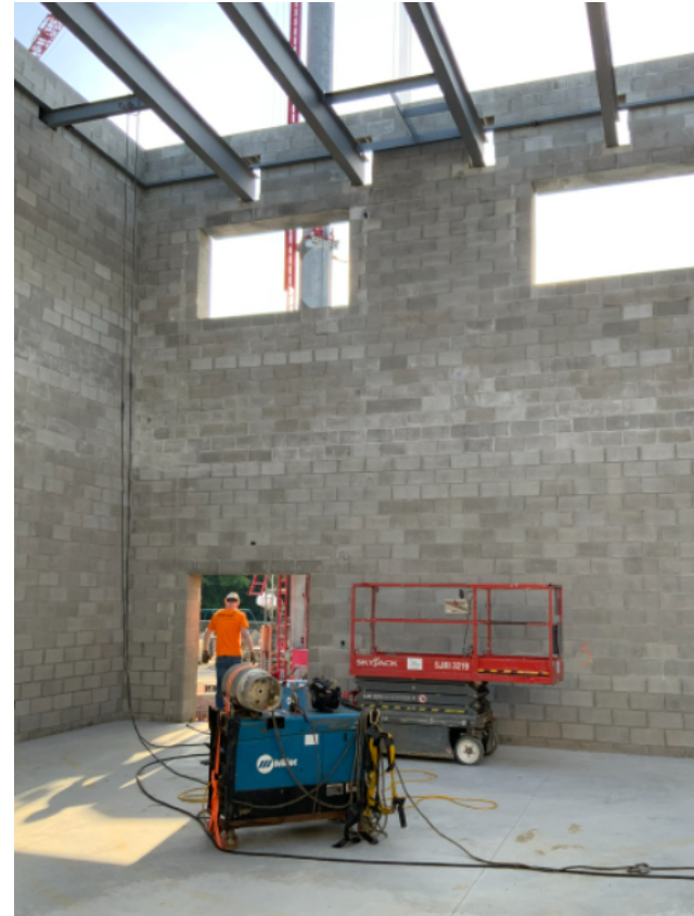
Structural Steel detailing throughout the addition
