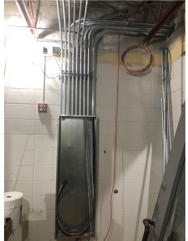
Tub for new Power Distribution Panel RP-L is installed in Storage Room near school office area.
