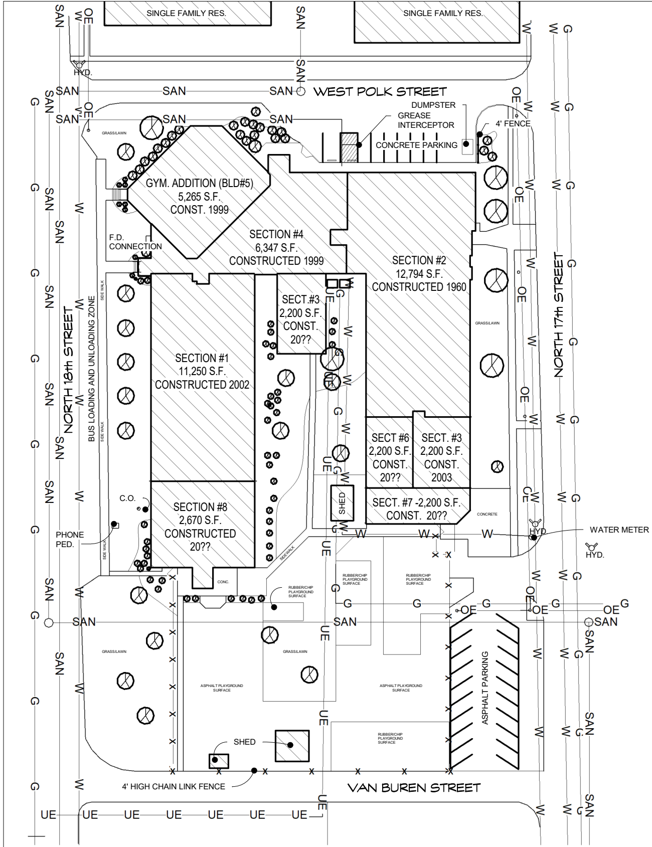
1 SAFETY REFERENCE SITE PLAN 1" = 60'-0"
