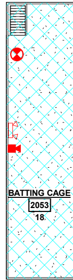
② SECTION #4 UPPER LEVEL PLAN 1/32" = 1'-0"
