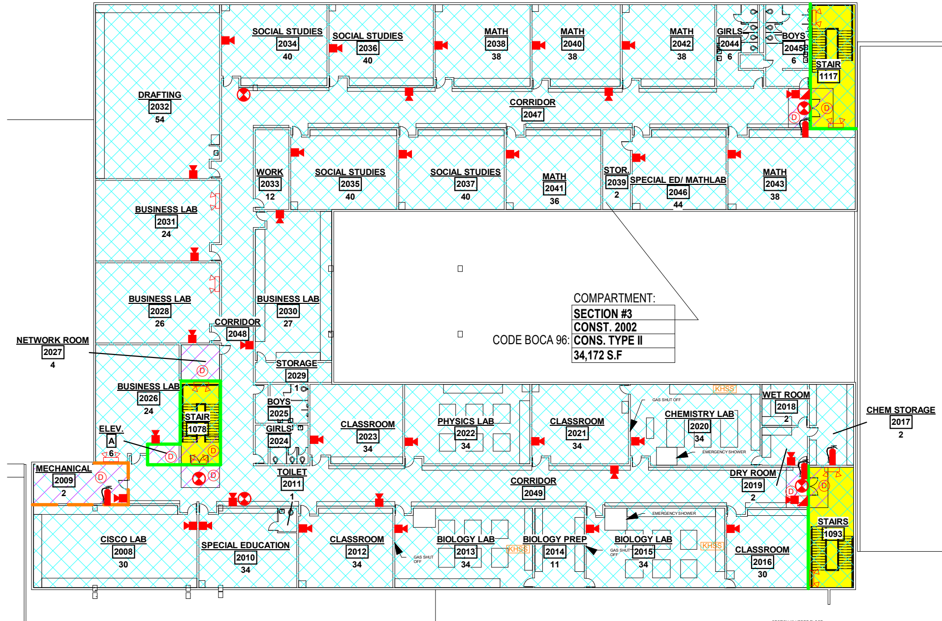
① SECTION #3 UPPER FLOOR PLAN 1/32" = 1'-0"
