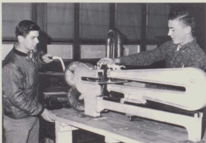
Cutting sheet metal on the ring and circle shears Mogan and Jim Moorehead.
