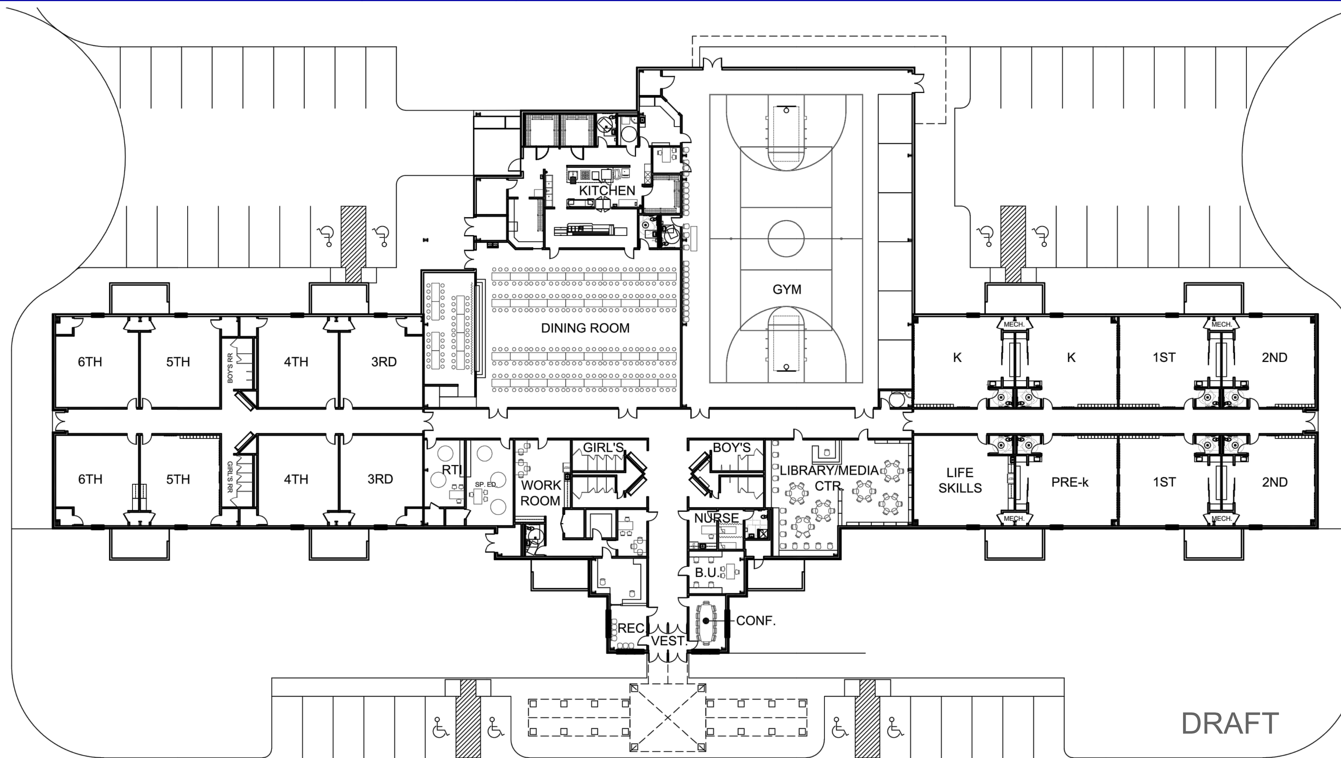
SCHEMATIC FLOOR PLAN
